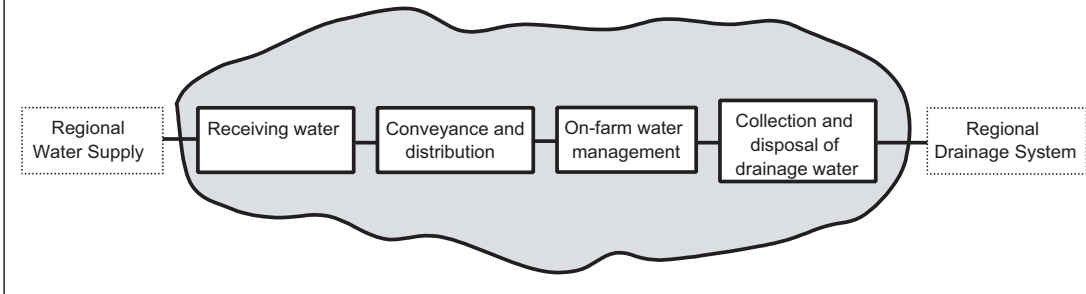
FIGURE 2 Example of a water management system within an irrigation district
