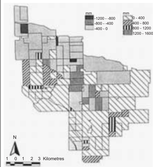
FIGURE 6 Annual recharge to groundwater in Panoche Water District
