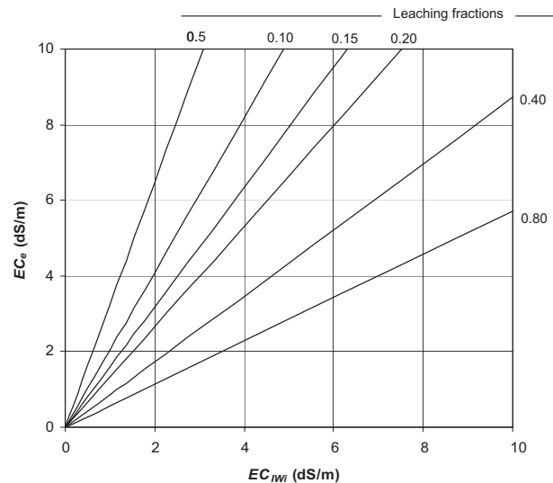
FIGURE 23 Assessment of leaching fraction in relation to the salinity of the infiltrated water
