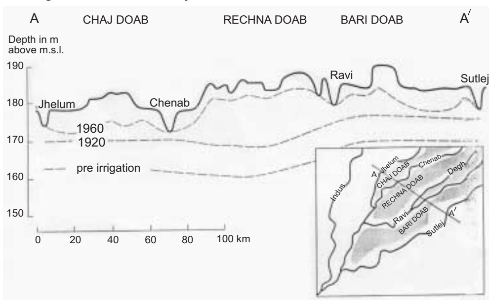
FIGURE 1 Rise of the groundwater table in Punjab, Pakistan
