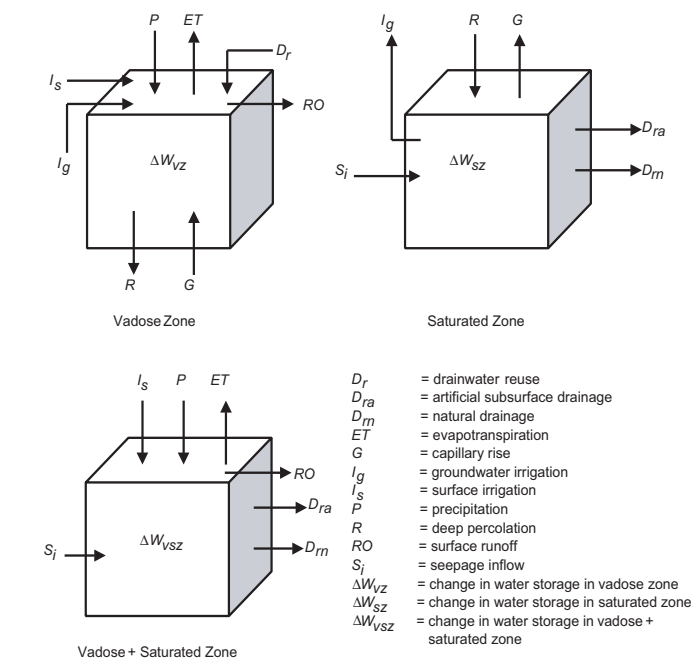
FIGURE 15 Hydrologic balance in the vadose and saturated zones, and in a combination of vadose and saturated zones
