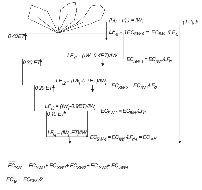
FIGURE A4.2 Calculation of rootzone salinity of five successive depths
