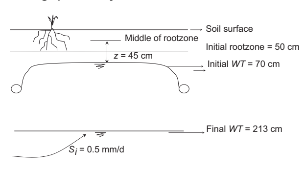
FIGURE 32 Change in water table during the winter season in the drainage pilot study area
