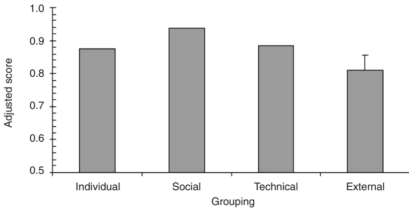
Fig. 13.7. Adjusted scores of the aggregated drivers associated with the development of bright spots of cases that focused on community-based upstream activities in India, Latin America and Africa. Vertical bar represents the least significant difference ( LSD_{0.05} ) between treatment means.
