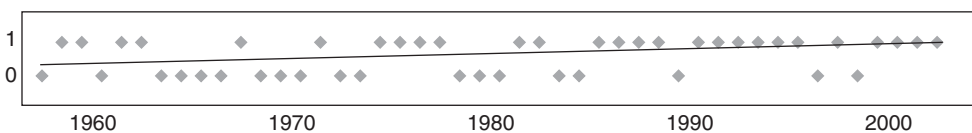
Fig. 3.6. Dry spells in the Makanya catchment. Change in dry spell frequency, 1960 to 2000.
