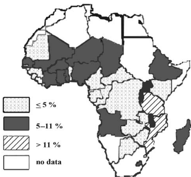
Fig. 5.1. Economic cost of NPK depletion at a national level as a percentage of the Agricultural Gross Domestic Product; categories of percentages are shown in different shades of grey (source: Drechsel et al. , 2001).
