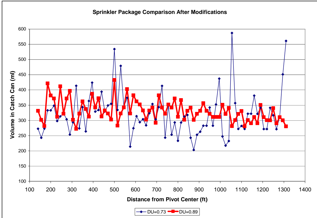
Figure 11. Catch can volumes from pivot center to edge of field (non-weighted)
