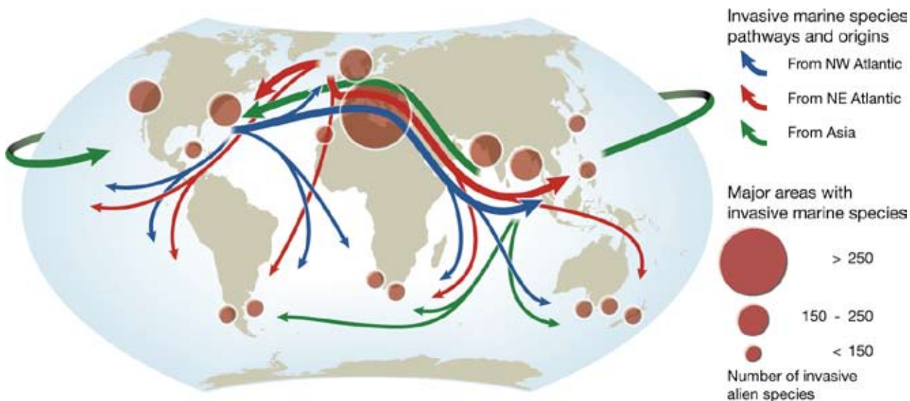
Figure 28. The major pathways and origins of invasive or exotic species infestations in the marine environment. These patterns are strikingly concurrent with major shipping routes.
