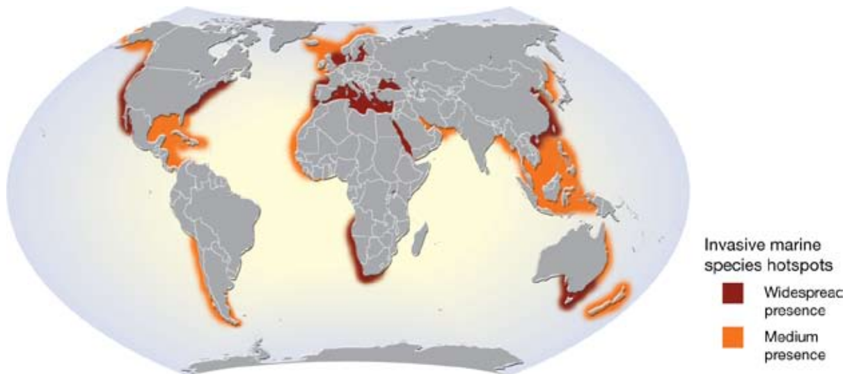
Figure 27. The locations of major problem areas for invasive species infestations or occurrence of exotic species in the marine environment. The impacted areas are concurrent with the areas subjected to the worst pollution, the most intensive fisheries and bottom trawling, and major shipping routes.
