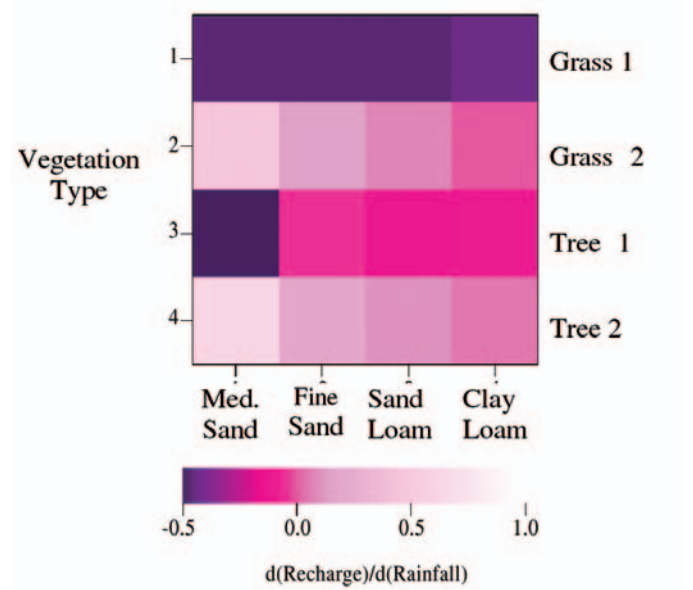
Figure 3. Simulated change in recharge per unit change in rainfall under a double- \text{CO}_2 climate change scenario in Western Australia (Green et al. 1997b). Grasses 1 and 2 are perennial grasses and Trees 1 and 2 represent pine and eucalyptus canopies with different model parameters for optimal temperature ranges, carbon assimilation, stomatal conductance, etc.
