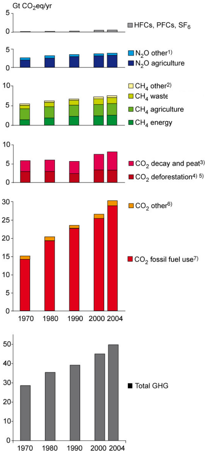
Figure SPM 1: Global Warming Potential (GWP) weighted global greenhouse gas emissions
