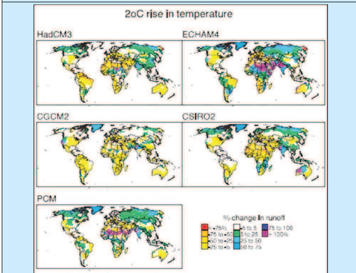
Figure 3.2 Changes in runoff with five different climate models
